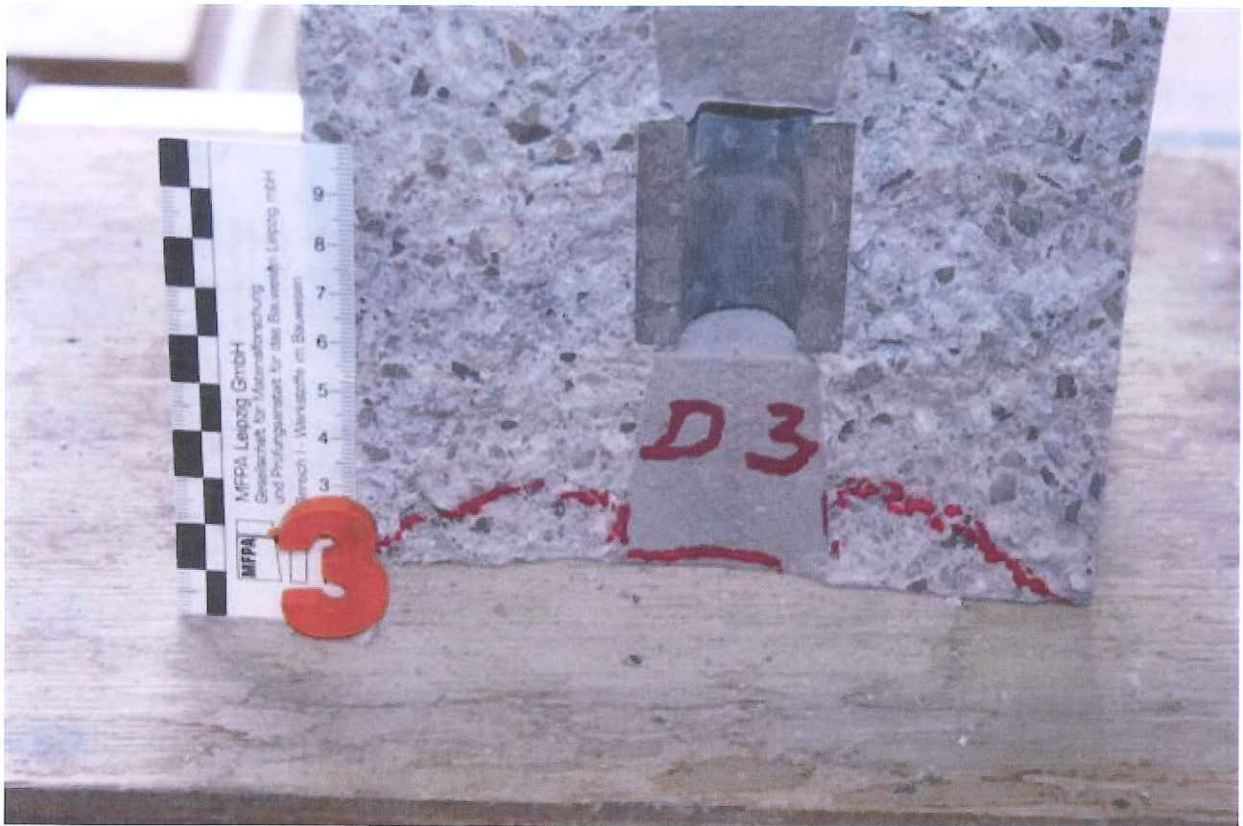
Photo 3: Series D 'FRANK' fibre-reinforced concrete distance tubes – MR 22 each sealed with one 5 cm sealing cone FBVK22T50, sample 3
